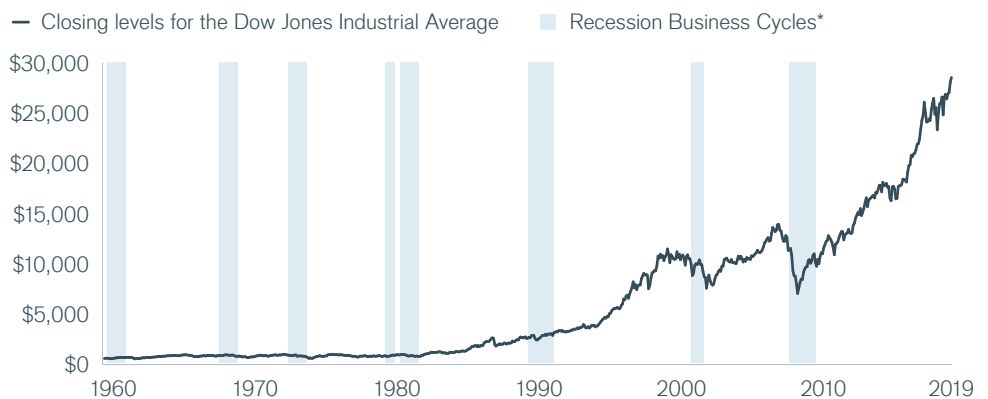
Monthly closing levels for the Dow Jones Industrial Average from 4/29/60 - 12/31/19
